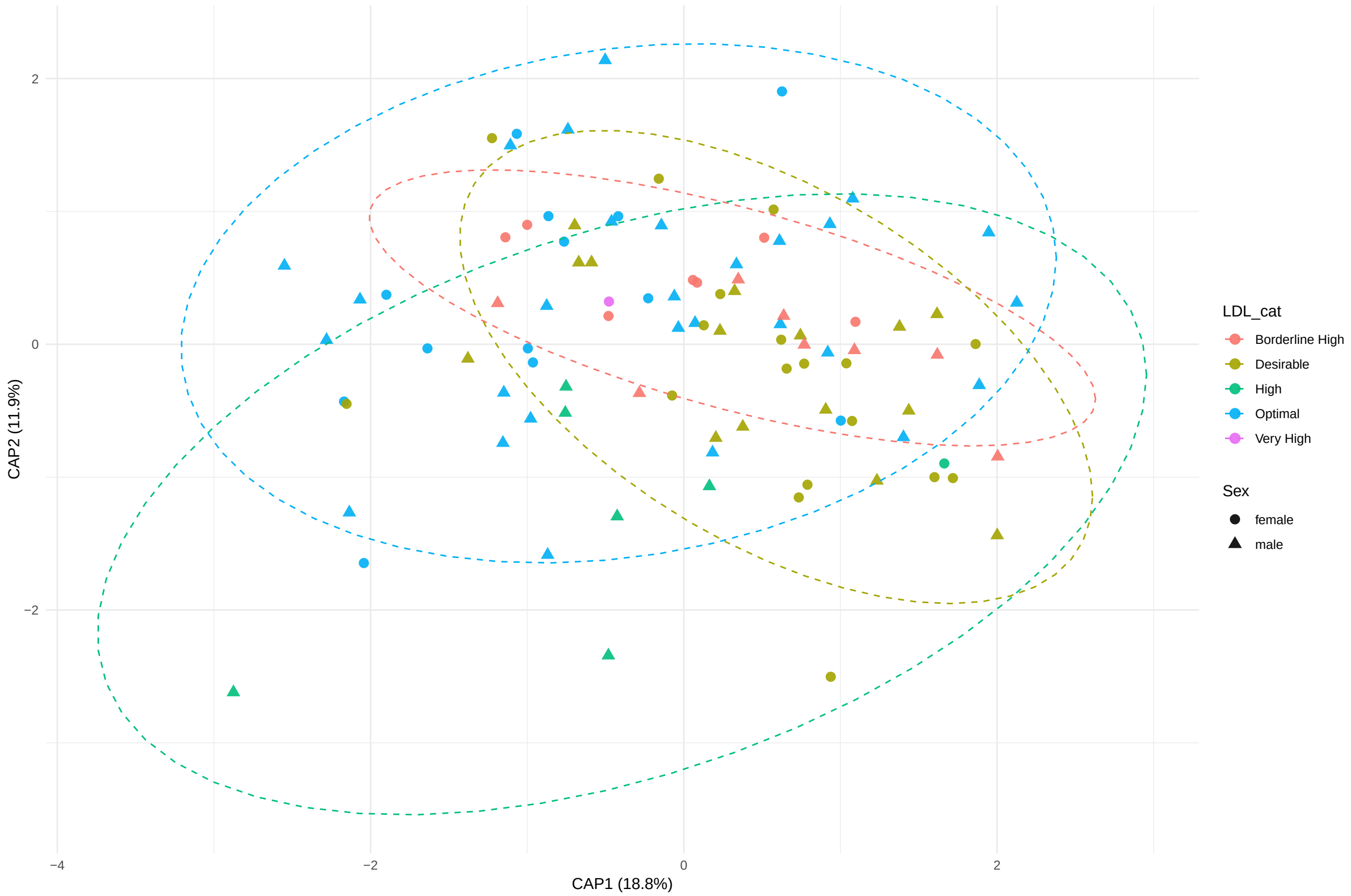
CAP Ordination by Multiple Variables adonis R^2 = 0.17 , p = 0.395
